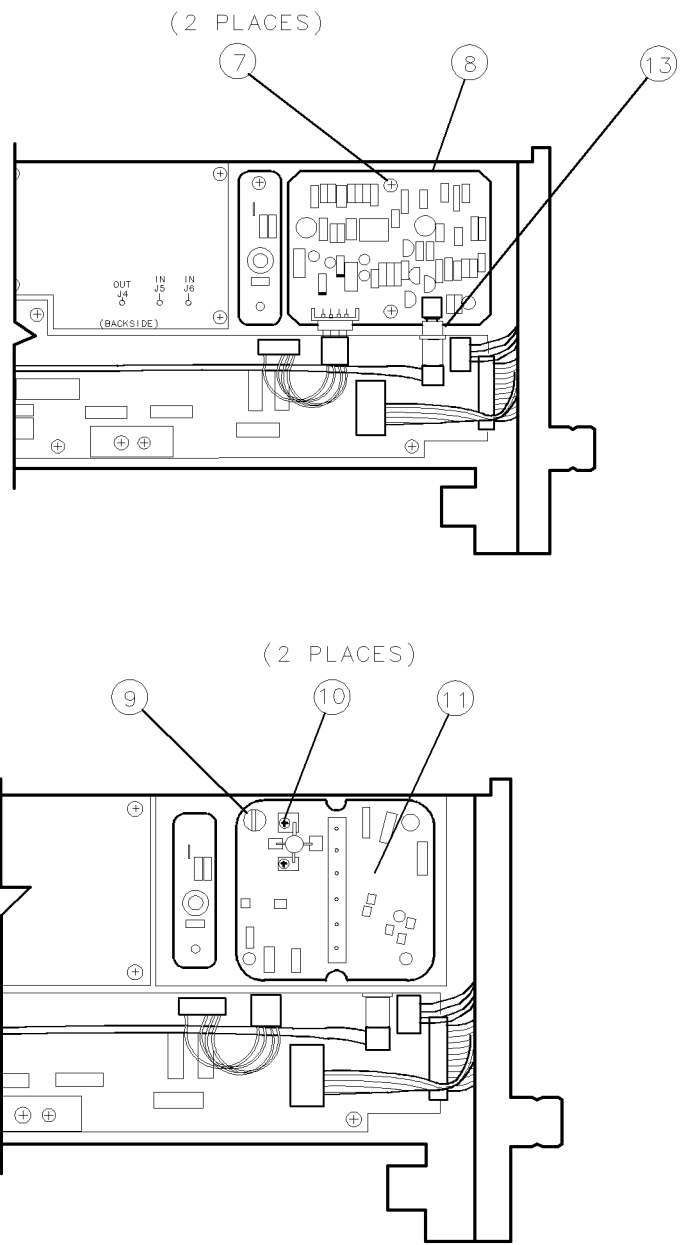
Figure 9-14. A5 VCO Sampler Removal/Replacement (2 of 3)
