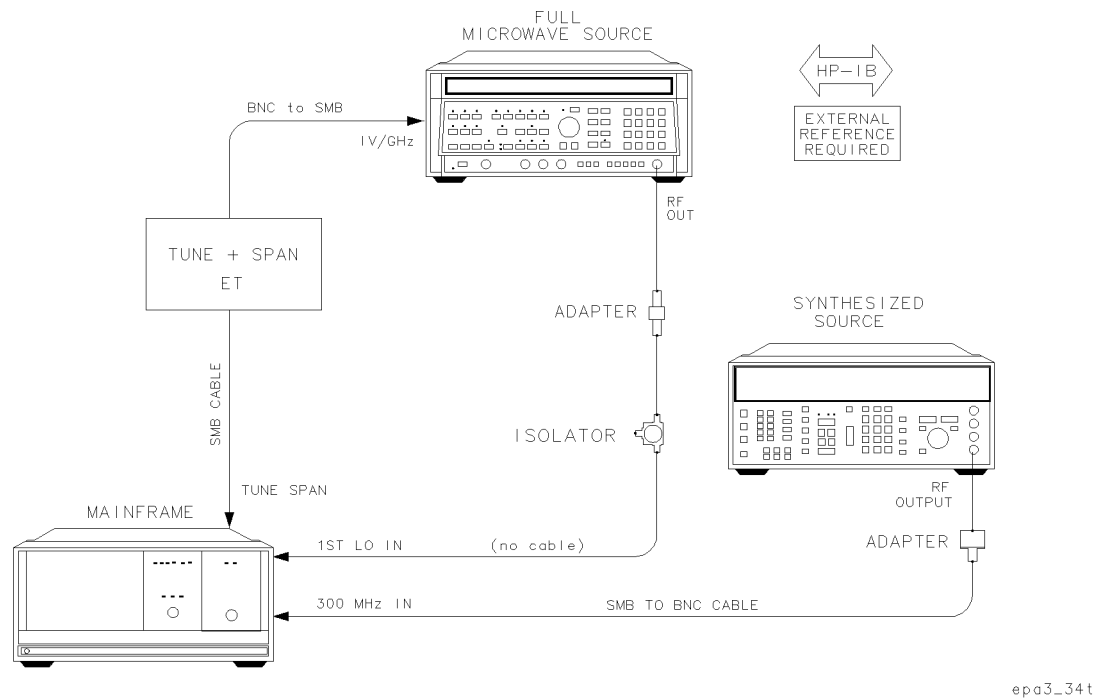
Figure 8-22. Equipment Setup for Test 20. Diagnostics (2 of 2)
