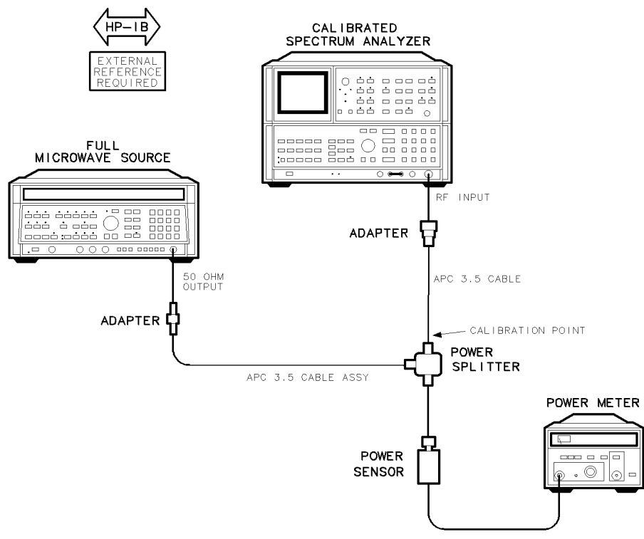
Figure 6-9. Spectrum Analyzer RF Calibration Test Setup
