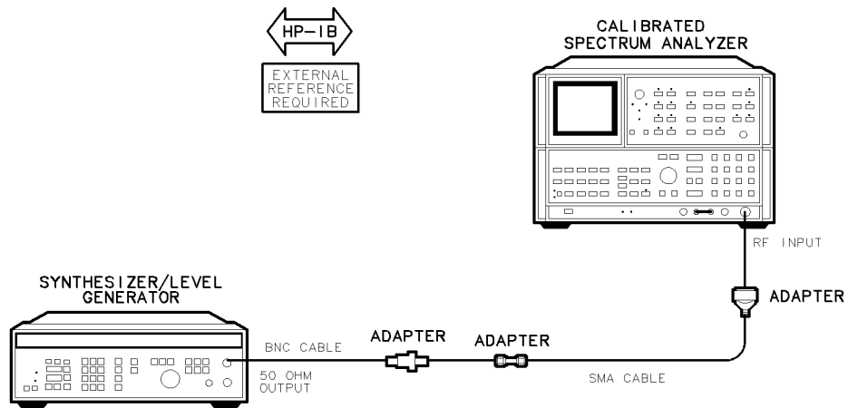
Figure 6-8. Spectrum Analyzer IF Calibration Test Setup
