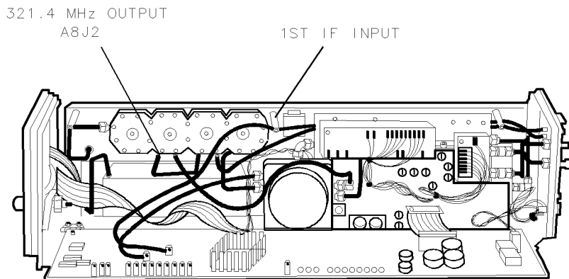
Figure 7-55. Locations for Adjustment 26. Noise Figure 2nd Converter
