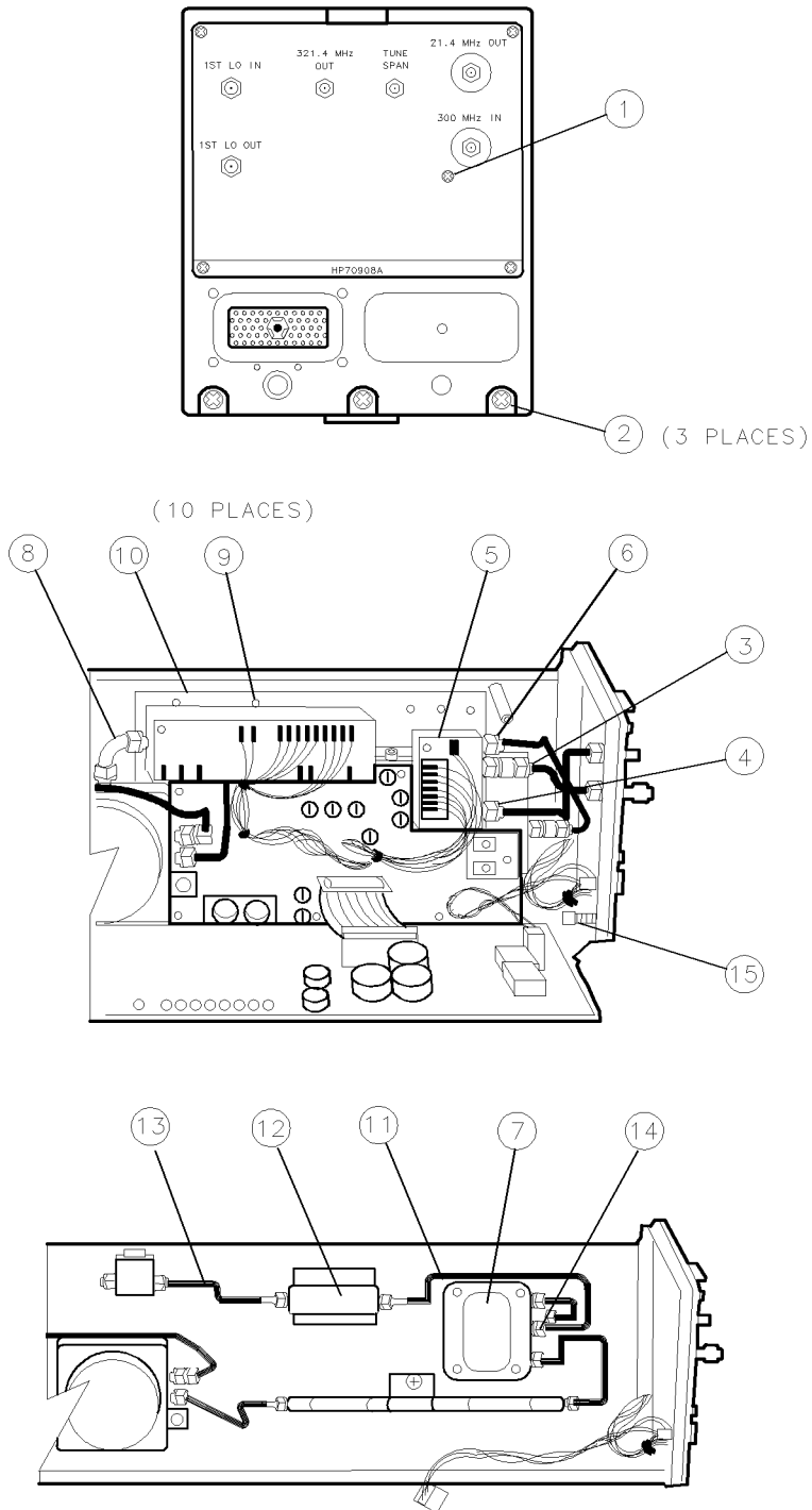
Figure 9-28. A16 Low Pass Filter Removal/Replacement
