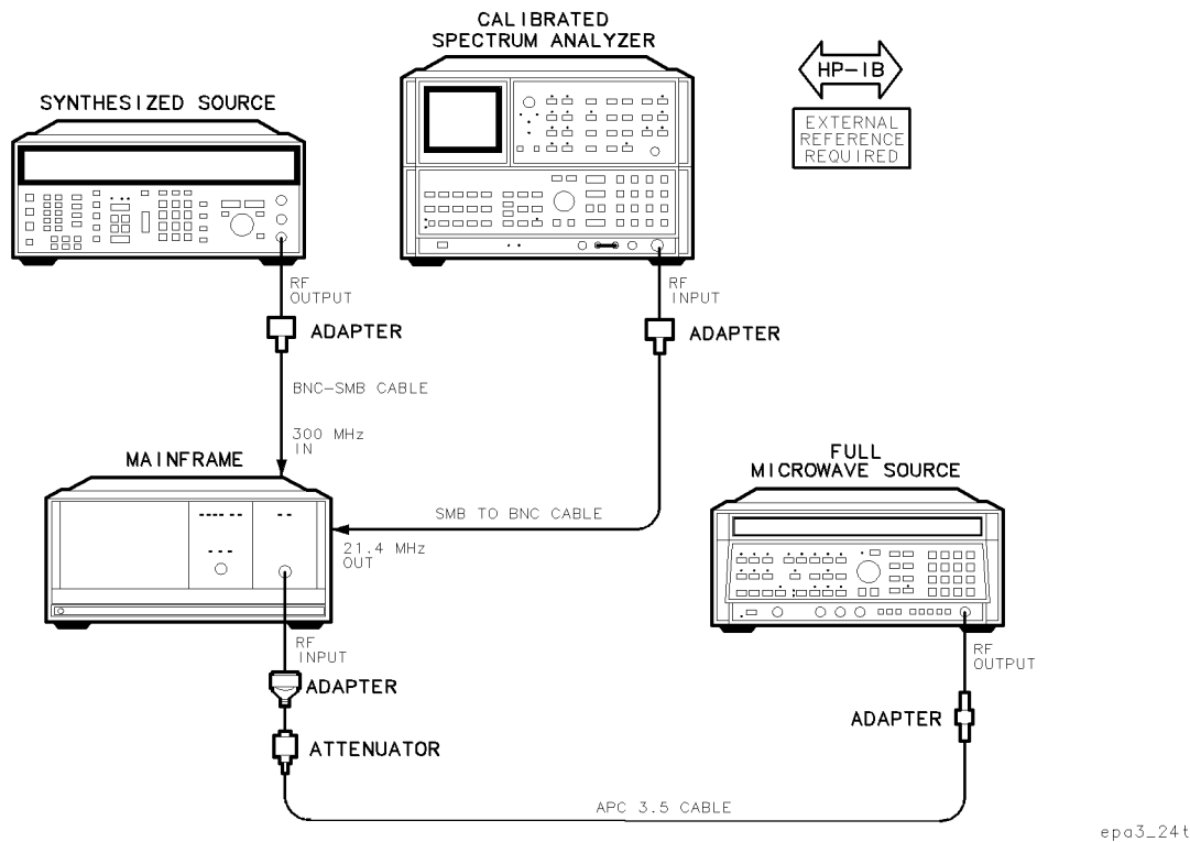
Figure 8-13. Equipment Setup for Test 12. IF Sub-Harmonics
