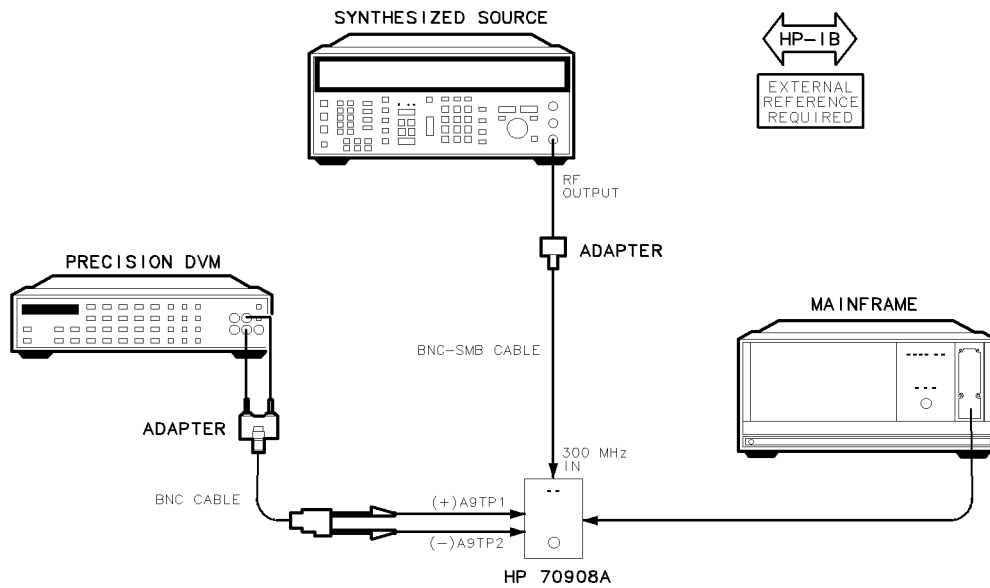
Figure 7-33. Equipment Setup for Adjustment 16. Search Oscillator Square Wave Min/Max
