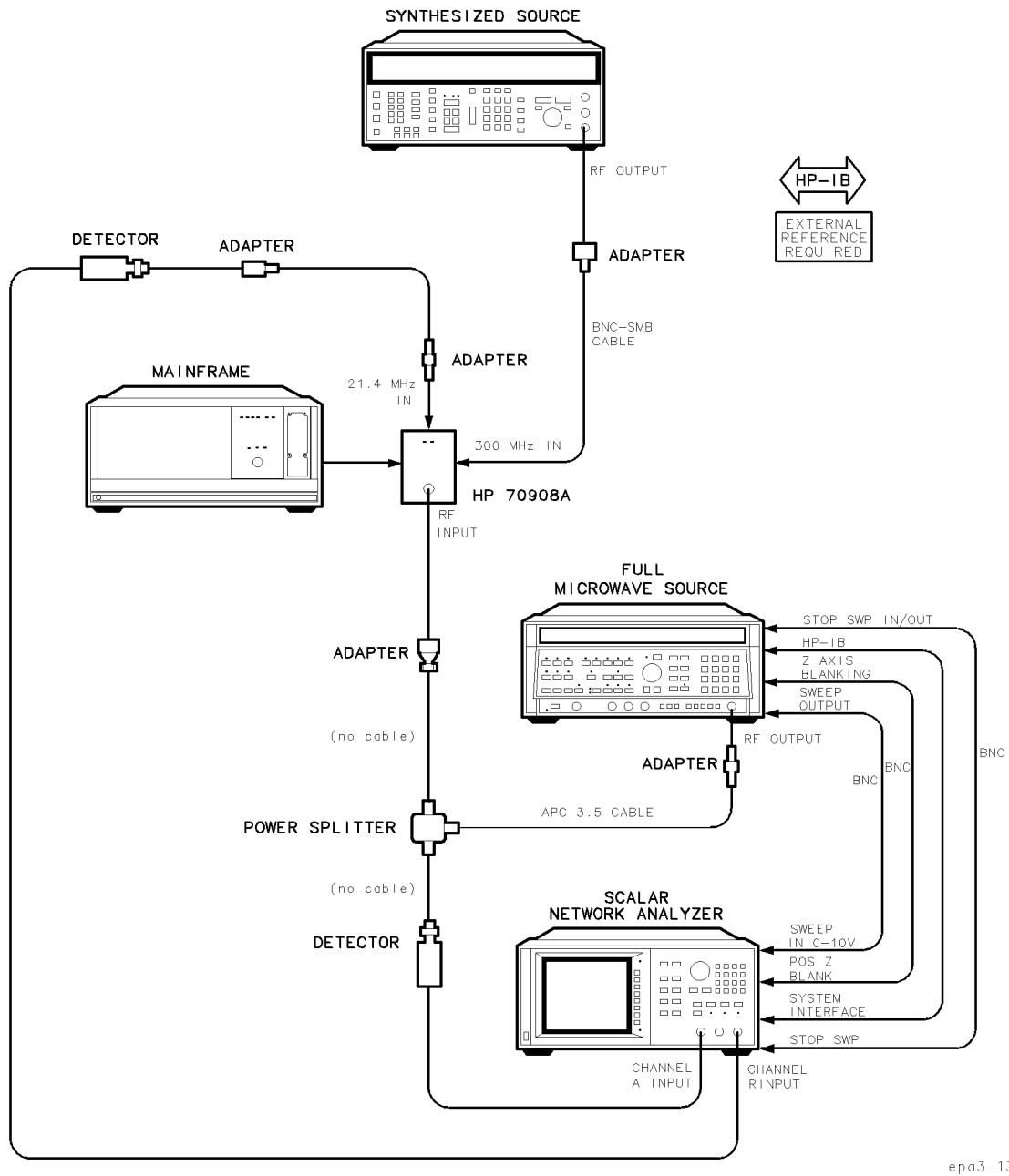
Figure 8-2. Equipment Setup for Test 01. Flatness
