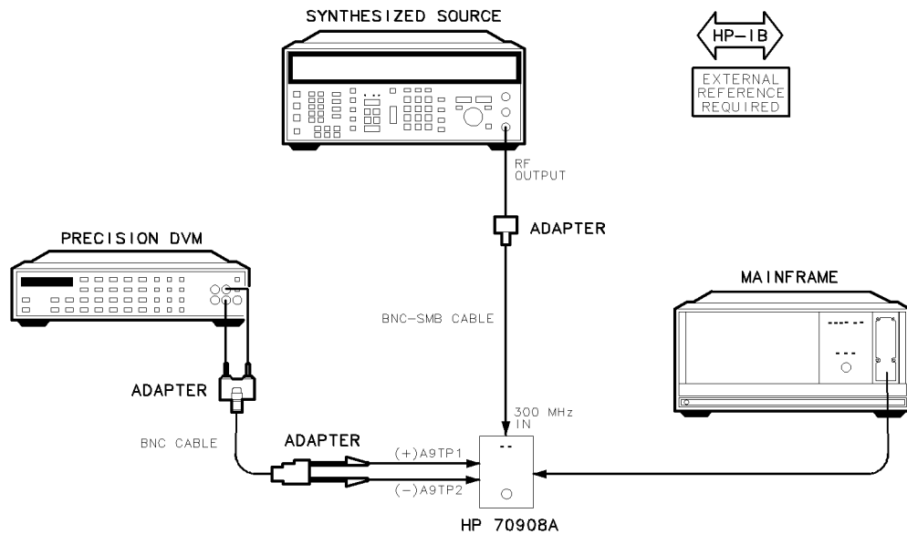
Figure 7-39. Equipment Setup for Adjustment 19. VCO Tune Range Preliminary Check
