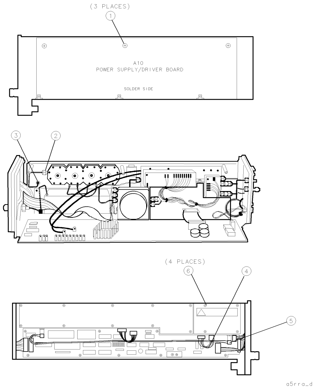
Figure 9-13. A5 VCO Sampler Removal/Replacement (1 of 3)
