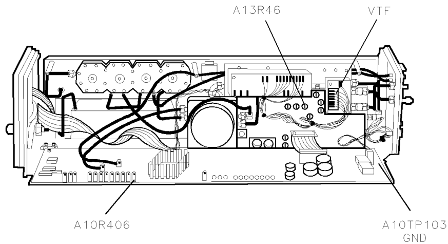
Figure 7-11. Locations for Adjustment 05. LOLA Tuned Filter
