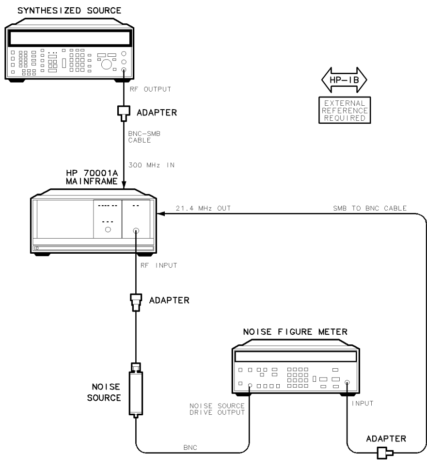
Figure 8-31. Equipment Setup for Test 29. Noise Figure
