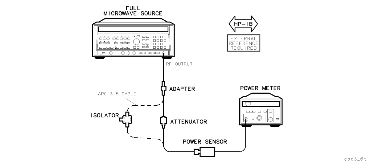
Figure 6-6. Microwave Source Calibration Test Setup
