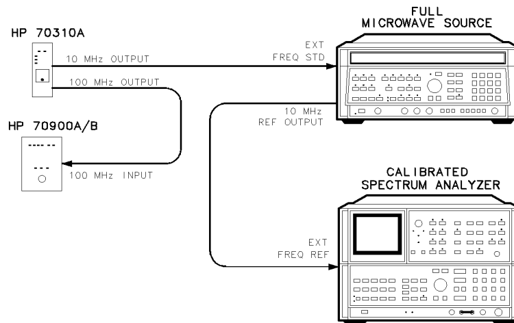
Figure 6-3. Using an HP 70310A Precision Frequency Reference
