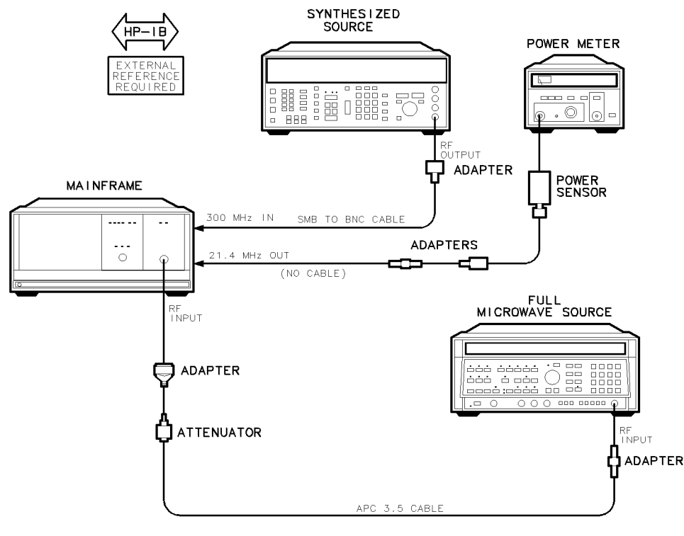
Figure 8-18. Equipment Setup for Test 17. Step Gain
