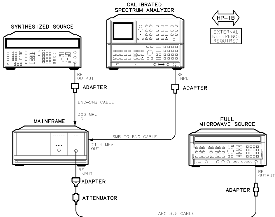
Figure 8-15. Equipment Setup for Test 14. Miscellaneous Residual Responses
