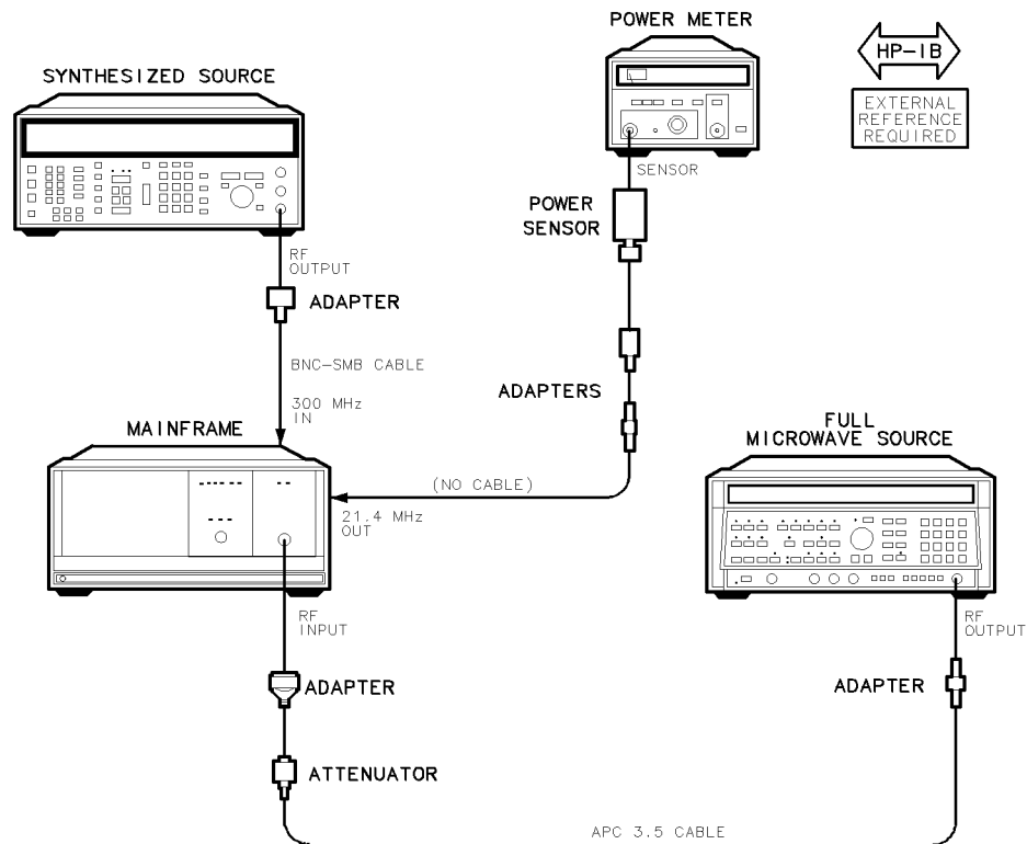
Figure 8-19. Equipment Setup for Test 18. Gain Compression
