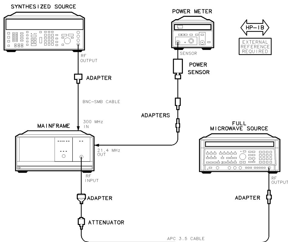
Figure 7-56. Equipment Setup for Adjustment 27. 21.4 MHz IF Frequency Response
