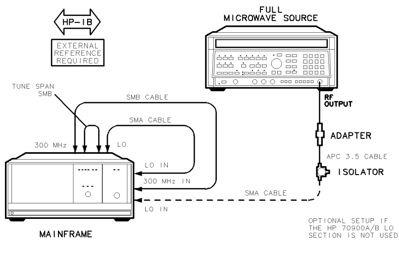
Figure 8-5. Equipment Setup for Test 04. Front Panel LEDs
