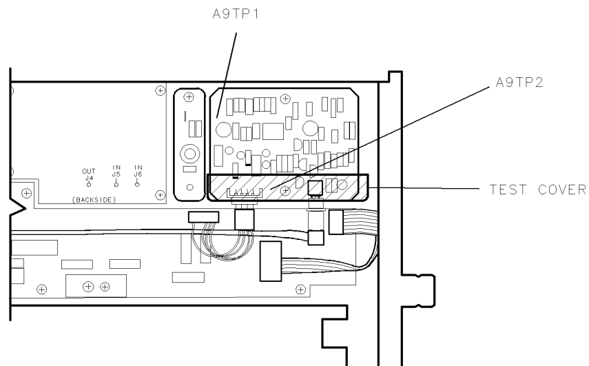
Figure 7-34. Locations for Adjustment 16. Search Oscillator Square Wave Min/Max
