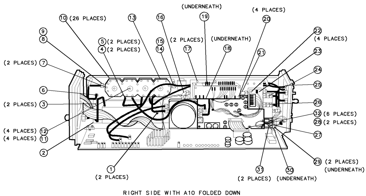
Figure 10-11. Overall Parts Identification Listing, Right Side View, A10 Power Supply/Driver Facing Down, and Cover Removed
