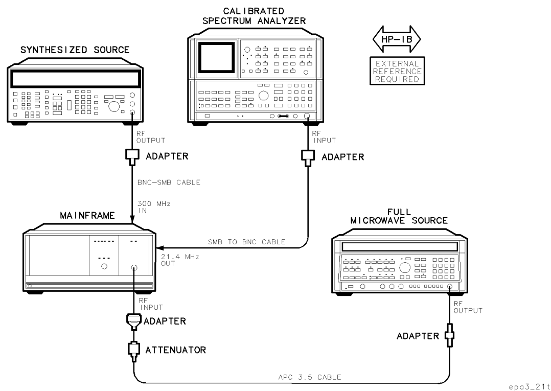
Figure 8-10. Equipment Setup for Test 09. Image Rejection
