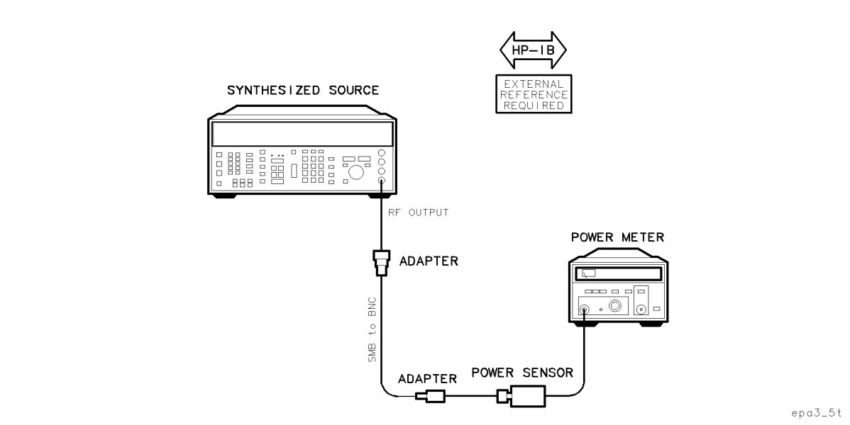
Figure 6-5. Synthesized Source Calibration Test Setup
